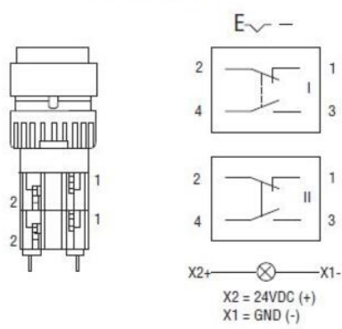
Wiring diagram
