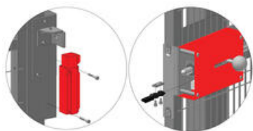
Latch lock
