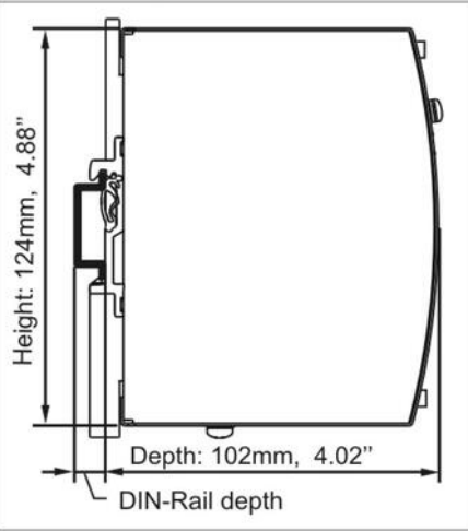
Fig. 19-2 Side view
