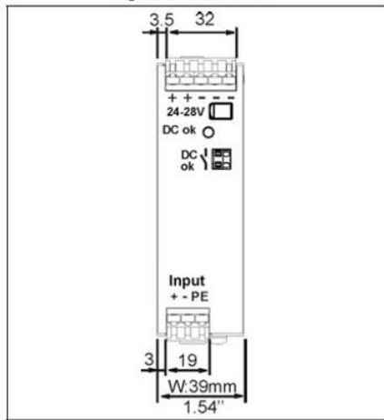
Fig. 22-1 Front view
