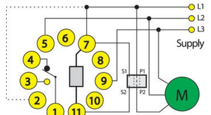
Example 2: With current transformer. (motor current bigger than 6 A)
