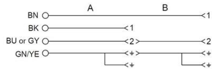
ELECTRICAL DIAGRAM - 00
