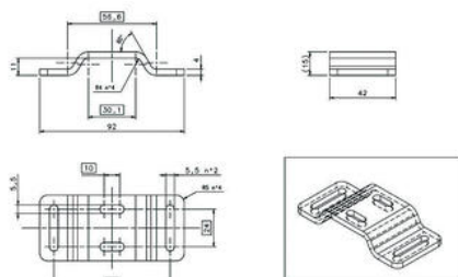
Bottom fixing bracket mounting
