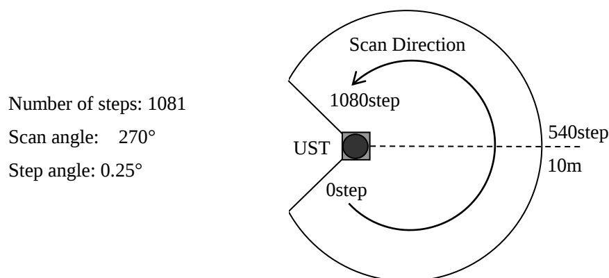
Fig.1 Detection Area
