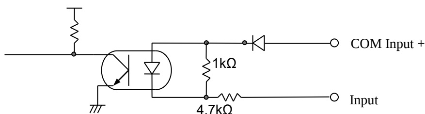
Fig.7 Input circuit
