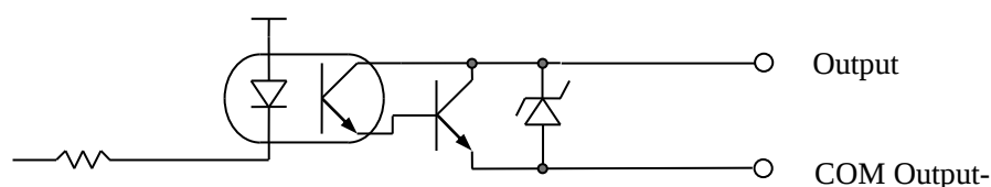
Fig.8 Output circuit
